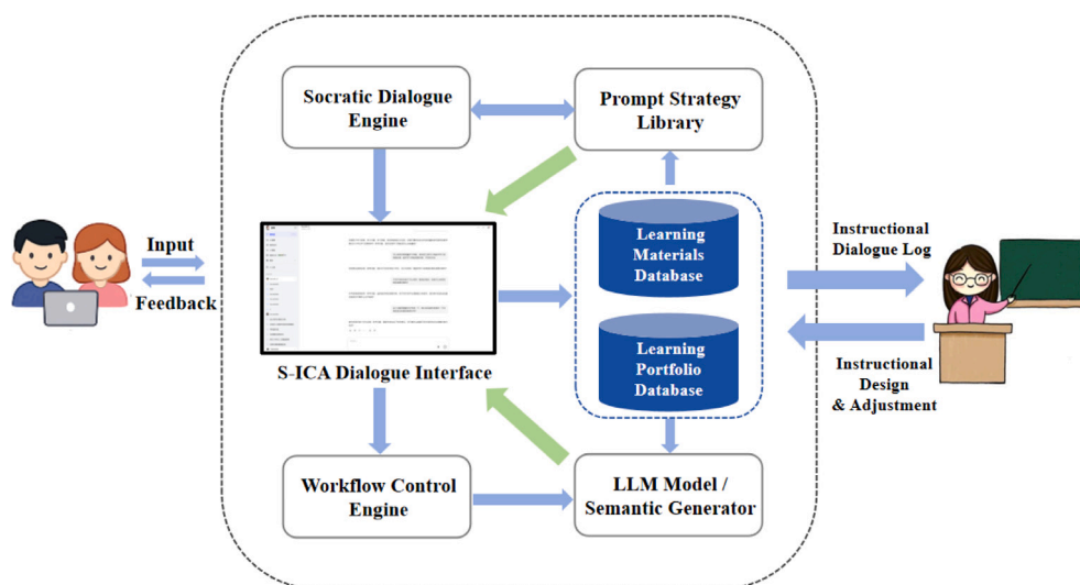
Fig. 1. System architecture of S-ICA.
